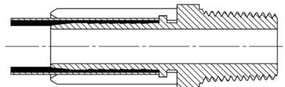
Crimped Fitting on Hose
